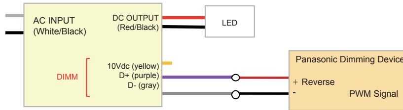
Wiring Diagram
